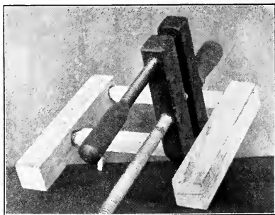
Fig. 224—Handscrew at End of Rung
